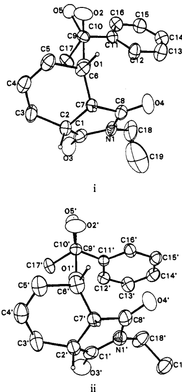
Figure 2. ORTEP diagram of cycloadduct ( \pm )- 17a of diene 5c with N -ethylmaleimide, showing the two independent rotamers (i and ii).
