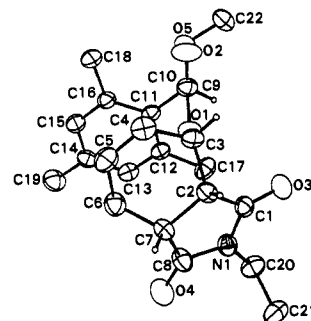
Figure 1. ORTEP diagram of the major cycloadduct ( \pm )- 8a of diene 5a with N -ethylmaleimide in toluene.
