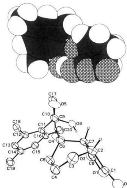
Figure 5. ORTEP diagram of the major cycloadduct ( \pm )- 19c of diene 5e with maleic anhydride in toluene, showing the hydrogen bonding (dotted line) between the \alpha -OH function and a carbonyl O of the dienophile moiety. Also shown is a space-filling model of this X-ray structure, which emphasizes the pocket-like environment of the hydrogen bond.
