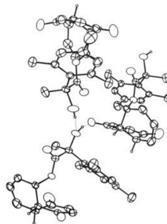
Figure 6. ORTEP diagram of the major cycloadduct ( \pm )- 19d of diene 5e with benzoquinone, showing the two independent rotamers that are linked through intermolecular hydrogen bonding (shown by dotted lines). Out of three rotamers shown here, the right-most one has R configuration of the chiral auxiliary, the other two, S , and the right-most and bottom rotamers are identical except for being enantiomeric.
