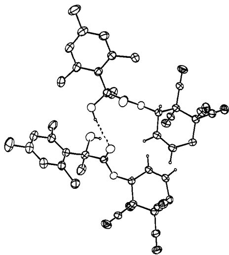
Figure 7. ORTEP diagram of the major cycloadduct ( \pm )- 21 of diene 5e with tetracyanoethylene, showing the two enantiomeric, but otherwise identical, rotamers that are linked through intermolecular hydrogen bonding (shown by dotted line). As shown, the upper structure has S configuration of the chiral auxiliary, the lower structure, R .
