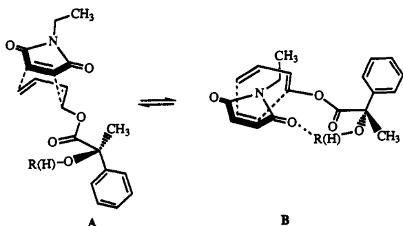
Figure 4. The two endo transition structures for reaction of diene 5c or 5d with N -ethylmaleimide.
