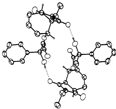
Figure 3. ORTEP diagram of cycloadduct ( \pm )- 16a of diene 5c with N -ethylmaleimide, showing the intermolecular hydrogen bonding between two enantiomeric, but otherwise identical, molecules in a head-to-tail fashion (shown by dotted lines). As shown, the left structure has S configuration of the chiral auxiliary, the right structure, R .
